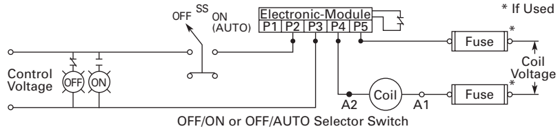
OFF/OA or OFF/AUTO Selector Switch
