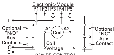
3-WIRE CONTROL
